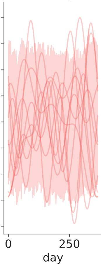
hierarchy=B
