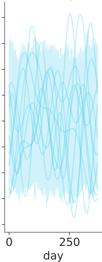
hierarchy=C
